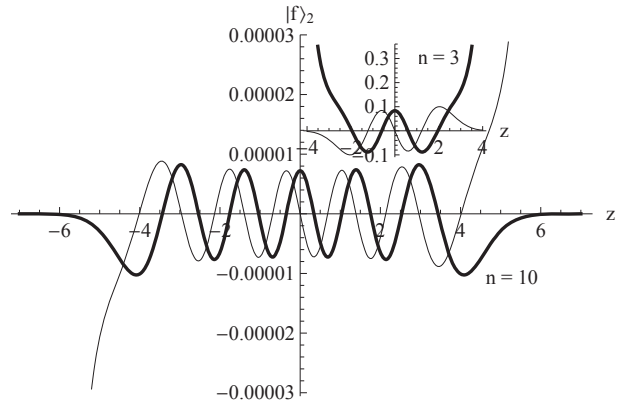
Fig. 1. Real (boldface curve) and imaginary (thin curve) parts of the function |f\rangle_2 from (41) versus the deviation z for n = 10 and n = 3 (in the inset)
