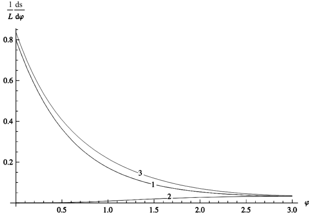
Fig. 2. Differential cross-section d\sigma/d\varphi in units of L versus the scattering angle \varphi for \lambda = 0.1 and \bar{k} = 0.8 . Curve 1 for the magnetic dipole moment of a nanomagnet perpendicular to the graphene plane, curve 2 for the magnetic dipole moment of a nanomagnet parallel to the incident electron beam in the graphene plane, curve 3 for the magnetic dipole moment of a nanomagnet parallel to the graphene plane and perpendicular to the incident electron beam in the graphene plane
