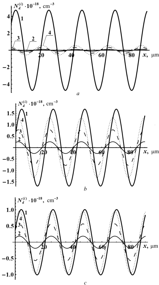
Fig. 1. Spatial redistributions of the chlorine (curve 1) and hydrogen (curves 2 to 4) impurities under the influence of an acoustic wave for various values of their average concentration N_{d0H} = 10^{20} (2), 3 \times 10^{20} , and 5 \times 10^{20} \text{ cm}^{-3} (4) and at various temperatures T = 300 (a), 600 (b), and 900 K (c)
