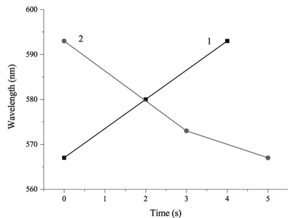
Fig. 6. Kinetics of the direct (curve 1) and reverse (curve 2) phototuning of the lasing wavelength of the induced CLC obtained, respectively, by using violet (curve 1) and green (curve 2) LEDs
