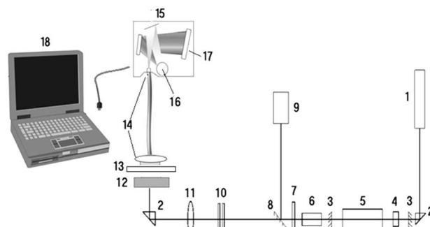
Fig. 1. Scheme of the laser setup: He-Ne laser (1), rotating prism (2), resonator mirrors (3), Q-modulator (4), active element of a solid-state laser (5), frequency doublers (6), filter (7), half mirror (8), calorimeter (9), neutral filters (10), lens (11), dye-doped CLC (12), filter (13), lens with optical fiber (14), spectrometer Ocean Optics USB 2000 (15), diffraction grating (16), CCD matrix (17), computer (18)
