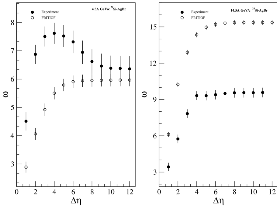
Fig. 6. Variation of the scaled variance with rapidity window for the interactions ^{28}\text{Si} with the AgBr target at 4.5A and 14.5A GeV/c for experimental and FRITIOF data
