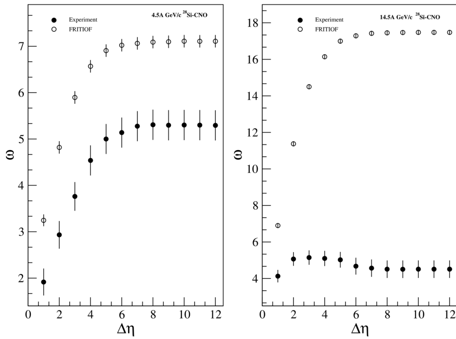
Fig. 5. Variation of the scaled variance with rapidity window for the interactions ^{28}\text{Si} with the CNO target at 4.5A and 14.5A GeV/c for experimental and FRITIOF data
