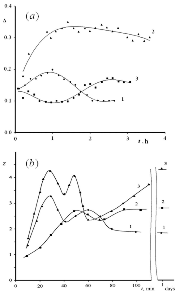
Fig. 9. Dependences of the coefficient of scattered light depolarization in water-glycerol solutions on the time interval spent after the preparation of the solution. The mole fraction of glycerol in the solution x = 0.031 (1), 0.035 (2), and 0.046 (3). The temperature is 10\text{ }^{\circ}\text{C} . Curve 3 corresponds to the concentration, at which the abnormal peak in the light scattering is observed (a). Angular asymmetry of the scattered light intensity as a function of time after the preparation of the aqueous glycerol solution by the ultrasonic mixing (b). The mole fraction of glycerol in the solution x = 0.047 (1), 0.035 (2), and 0.056 (3). The figures were taken with permission from work [30]
