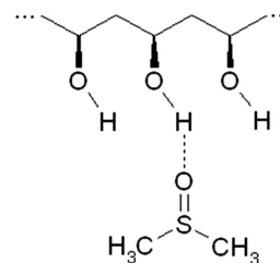
Fig. 2. Diagram of hydrogen bond formation between a monomer of a PVA macromolecule and a DMSO molecule
