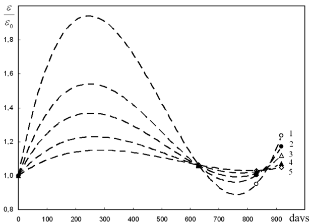
Fig. 3. Dependences of the relative dielectric permittivity on the preparation time for the PVA solution in DMSO with a concentration of 5 wt.% at various frequencies: 2 (1), 4 (2), 6 (3), 10 (4), and 200 kHz (5). Dashed curves demonstrate approximations by formula (3)
