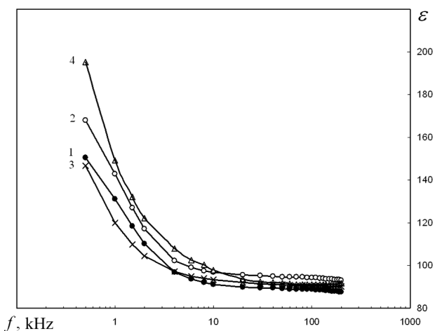
Fig. 4. Frequency dependences of the dielectric permittivity of the PVA solution in DMSO with a concentration of 5 wt.% measured in 0 (1), 628 (2), 831 (3), and 918 days (4) after the preparation of the solution
