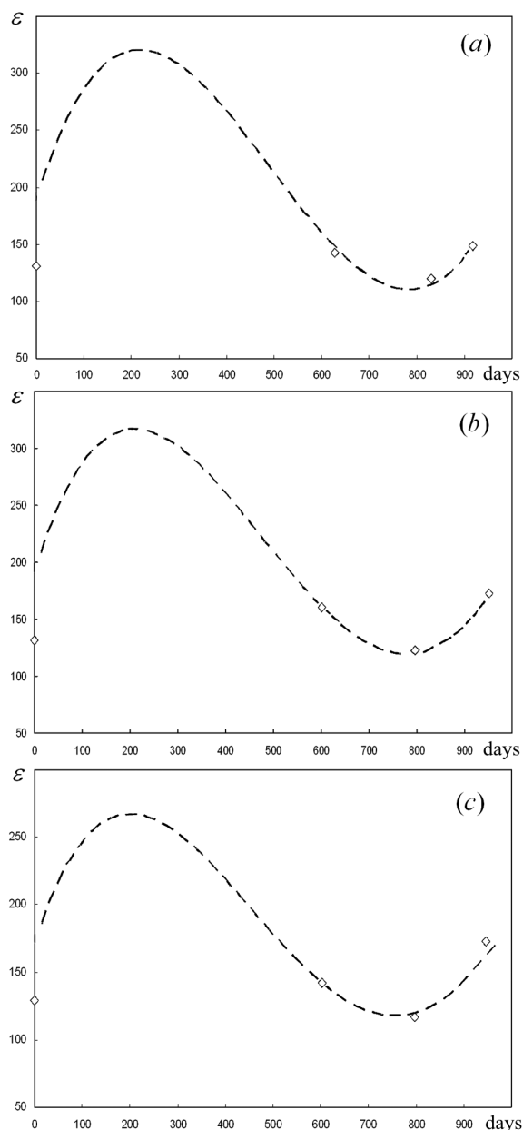
Fig. 10. Experimental data for the dielectric permittivity of PVA solutions in DMSO with concentrations 5 (a), 10 (b), and 15 wt.% (c) at a frequency of 1 kHz (diamonds) and their approximations by formula (3) (dashed curves)
