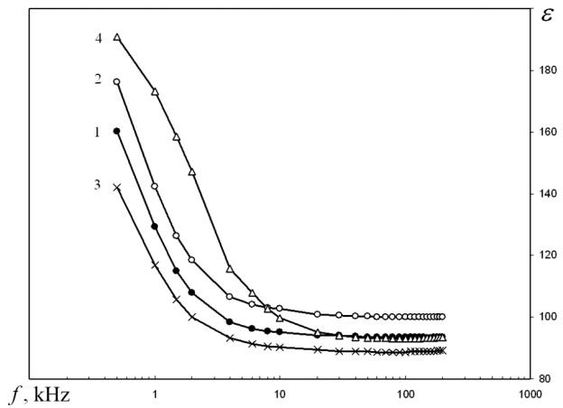
Fig. 8. Frequency dependences of the dielectric permittivity of the PVA solution in DMSO with a concentration of 15 wt.% measured 0 (1), 603 (2), 798 (3), and 947 days (4) after the preparation of the solution
