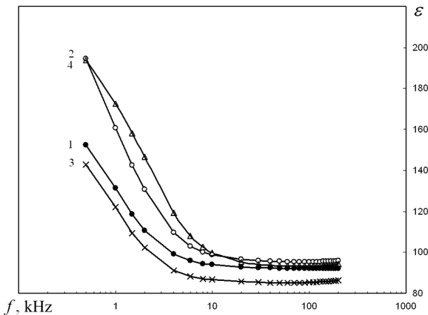
Fig. 6. Frequency dependences of the dielectric permittivity of the PVA solution in DMSO with a concentration of 10 wt.% measured in 0 (1), 601 (2), 796 (3), and 952 days (4) after the preparation of the solution
