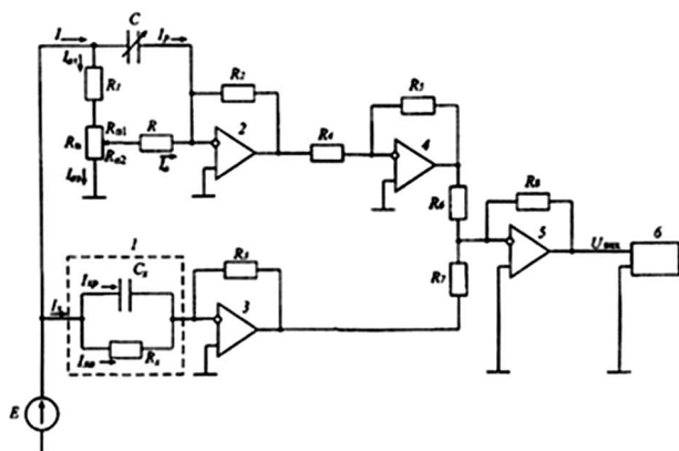
Fig. 1. Circuit diagram of the electronic bridge: the equivalent circuit of a measuring condenser (1), integrated operational amplifiers (2-5), millivoltmeter (6), variable condenser (C), calibrated potentiometer ( R_P ), sound generator (E)
