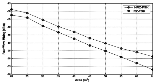
Fig. 4. FWM versus the effective area at different modulation formats
