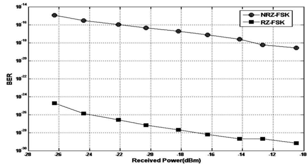
Fig. 6. BER versus the received power for different modulation types
