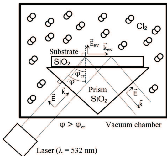
Fig. 1. Scheme of the experimental setup ( \vec{k}_{ev} and \vec{E}_{ev} are wave vector and the electric field strength of the evanescent wave, respectively, \varphi is the angle of incidence of the laser radiation on the lower surface of a quartz substrate, \varphi_{cr} is the critical angle)
