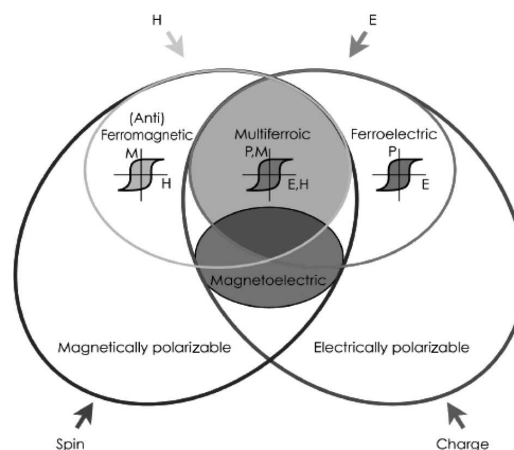
Fig. 2.1. Ferroics, multiferroics, and magnetoelectrics (reproduced from Ref. [3])
