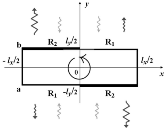
Fig. 1. Diagram (cross-section) of a heated rotating plate. The wide faces (a) and (b) are divided into two halves each that differ in the reflection coefficients ( R_1 and R_2 ) and TR intensities (arrows of different lengths aimed away from the plate). The arrows directed toward the plate represent the background radiation. The round arrow represents the plate rotation direction around the axis passing through the center of inertia
