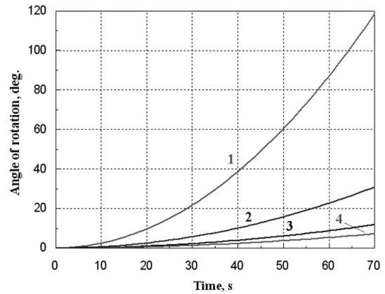
Fig. 2. Time dependence of the silicon plate rotation angle at the constant plate temperature T = 350 K and background temperature T_1 = 300 K: 1 and 3 – l_y = 0.1 mm and 1 mm, respectively, R_1 = 1, R_2 = 0 ; 2 and 4 – l_y = 0.1 mm and 1 mm, respectively, R_1 = 1, R_2 is the reflection coefficient of a polished plate
