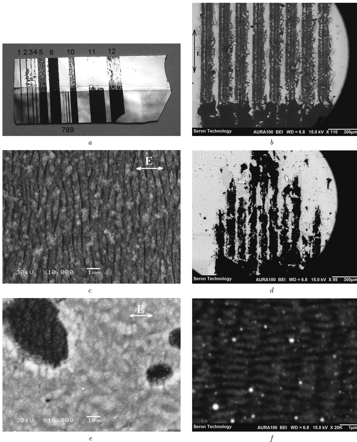
Fig. 1. Photo of the Au/(n-Si) composite sample surface (a) and SEM images of different areas of the Au/(n-Si) sample: overview of the sample with Au contact grid (group of lines 5) (b), laser-treated surface of Si without Au film (c), part of the Au contact grid (group of lines 11) (d), part of the Au film with incipient surface periodic structure (e), LIPSS on silicon with scattered gold NPs (f)
