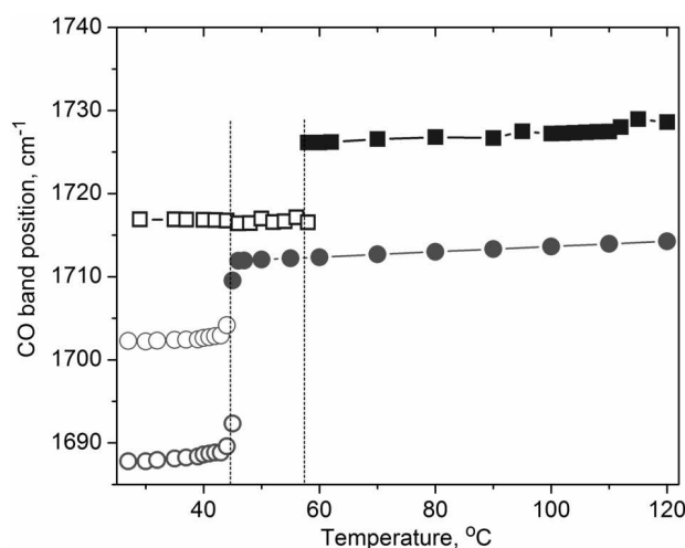
Fig. 7. Temperature evolution of the carbonyl stretching band /components position for the 1:1 kC12-CTAB binary complex (squares) and pristine kC12 (circles)
