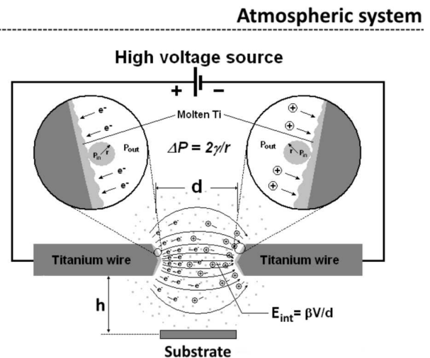
Fig. 1. Schematic diagram of the preparation of nanoparticles, by using the sparking process
