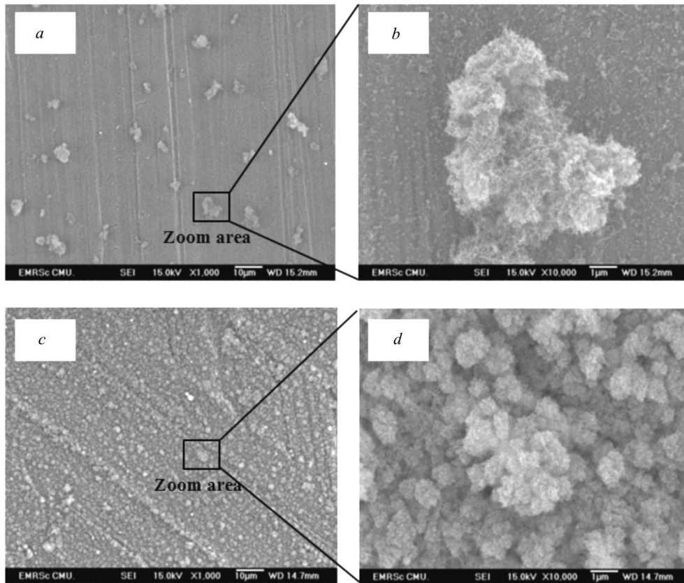
Fig. 3. SEM images of as-deposited thin films by sparking without external electric field (no E_{\text{ext}} ) (a–b), sparking with external electric field ( E_{\text{ext}} ) at 9 kV/cm for magnifications of 1,000 and 10,000, respectively, (c–d)
