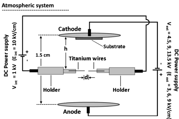
Fig. 2. Schematic diagram of the sparking apparatus
