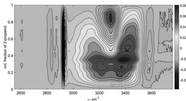
Fig. 2. ATR FTIR residual spectra
