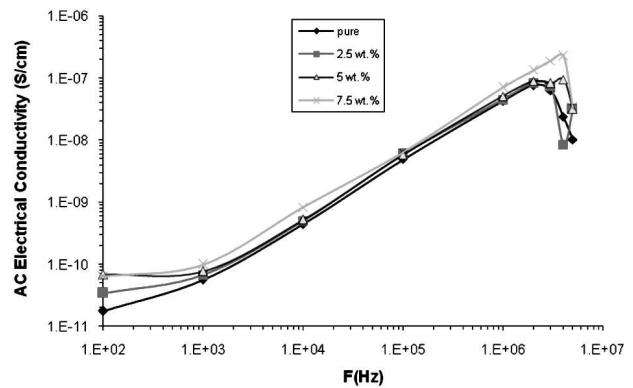
Fig. 3. Variation of the ac electrical conductivity for (PVA–PAA– \text{PbO}_2 ) nanocomposites with the frequency
