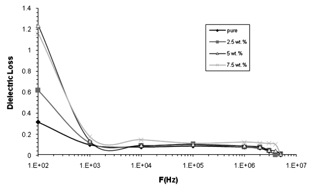
Fig. 2. Variation of the dielectric losses for (PVA–PAA– \text{PbO}_2 ) nanocomposites with the frequency
