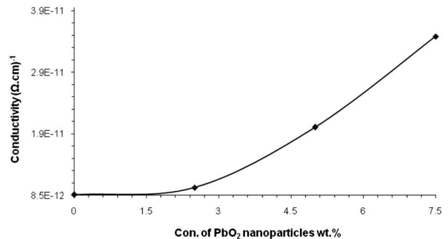
Fig. 4. Variation of the dc electrical conductivity for (PVA–PAA– \text{PbO}_2 ) nanocomposites with the concentration of \text{PbO}_2 nanoparticles
