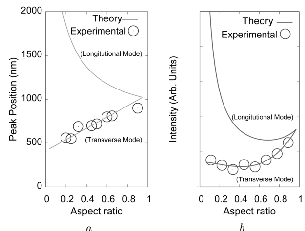
Fig. 2. Simulation shows variations in the SPR peak position ( a ) and the dependence of the peak intensity on the aspect ratio ( b ). Curves were generated for the fixed metal nanocluster size and surrounding medium
