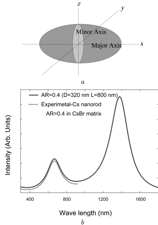
Fig. 1. Illustration of the geometrical shapes of the nanoparticle (ellipsoid) ( a ). The simulation shows SPR peaks of due to non-spherical cesium metal clusters in a cesium bromide medium (i.e. AR \neq 1 ) ( b ). The theoretical values agree well with the experimental curve
