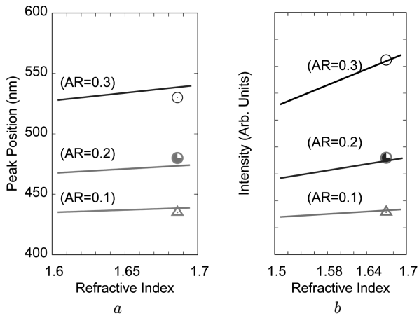
Fig. 3. Simulation shows a family of curves (different aspect ratios) exhibiting variations in SPR peak positions (triangle, filled circle, and circle for AR = 0.1, 0.2, and 0.3, respectively) (a) and peak intensities (triangle, filled circle, and circle for AR = 0.1, 0.2, and 0.3, respectively) with the refractive index of a surrounding medium (b)
