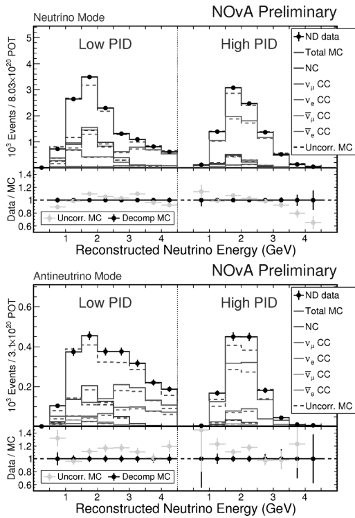
Fig. 4. ND selected \nu_e (top) and \bar{\nu}_e (bottom) reconstructed energy data (black dots), uncorrected simulation (dashed red) and data-driven correction (solid red). The selection is decomposed (broken down) into NC (blue), \nu_\mu/\bar{\nu}_\mu CC (dark/light green) and \nu_e/\bar{\nu}_e CC (light/dark magenta). Binned in two PID bins, which are correlated to lower and higher purities of \nu_e + \bar{\nu}_e
