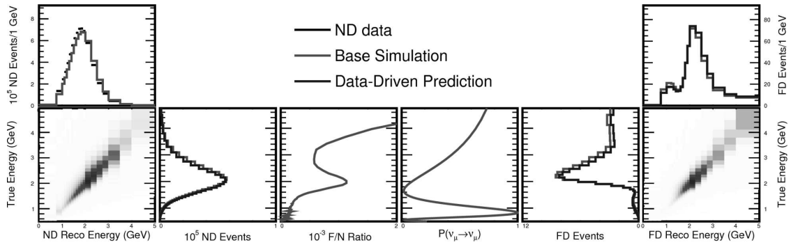
Fig. 1. Illustration of the NOvA’s F/N technique. From left to right: reconstructed to true \nu_\mu energy translation, F/N ratio, \nu_\mu \rightarrow \nu_\mu oscillation probability, true to reconstructed \nu_\mu energy restoration. Base simulation in red (light), ND data-driven corrected prediction in blue (dark)
