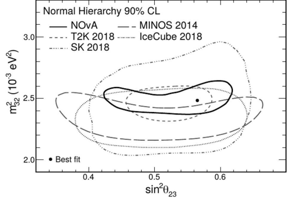
Fig. 6. Comparison of the allowed regions of \Delta m_{32}^2 vs. \sin^2 \theta_{23} parameter space at the 90% confidence level as obtained by recent experiments
