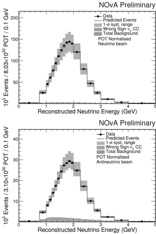
Fig. 2. ND selected \nu_\mu (top) and \bar{\nu}_\mu (bottom) reconstructed energies in data (black dots) and simulation (band). Each bin is normalized by its width
