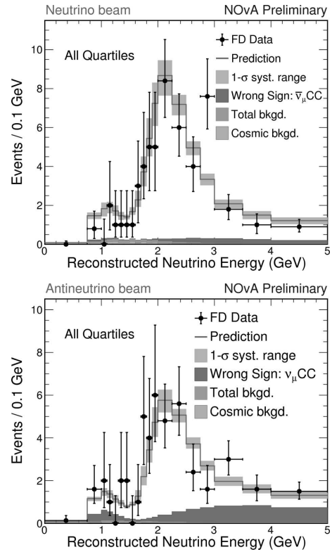
Fig. 3. FD data (black dots) selected \nu_\mu (top) and \bar{\nu}_\mu (bottom) candidates reconstructed energies compared to the best fit prediction (line) with 1\sigma systematics uncertainty range. Summed over all quartiles of the hadronic energy fraction
