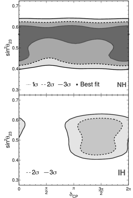
Fig. 7. 1, 2, and 3\sigma allowed regions of \sin^2 \theta_{23} vs. \delta_{\text{CP}} neutrino oscillation parameter space consistent with the \nu_e appearance and \nu_\mu disappearance data. The top panel corresponds to the case of normal hierarchy (NH) of neutrino masses ( \Delta m_{32}^2 > 0 ), the bottom one to the inverted hierarchy (IH, \Delta m_{32}^2 < 0 )
