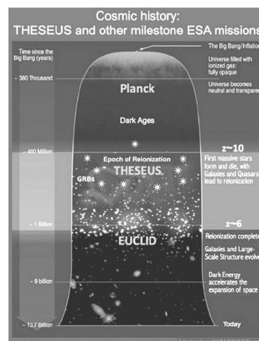
Fig. 1. Gamma-ray bursts in the cosmological context and the role of THESEUS (adapted from a picture by the NASA/WMAP Science team)
