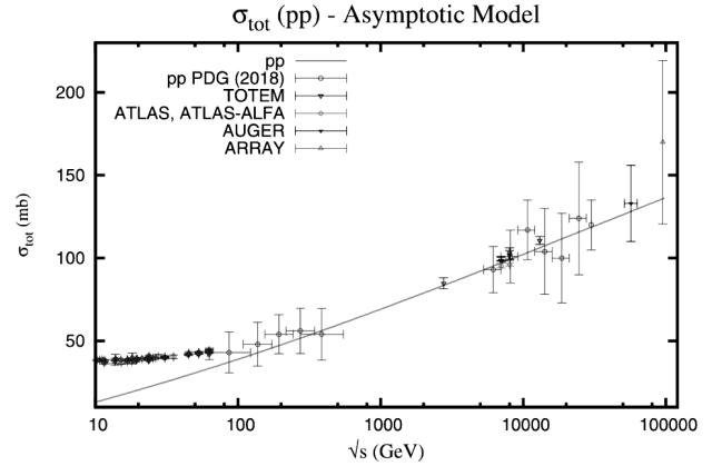
Fig. 1. ( pp total cross-section as a function of the center-of-mass-energy, including low-energy and cosmic rays data. The LHC data are explicitly identified (TOTEM and ATLAS Collaborations)
