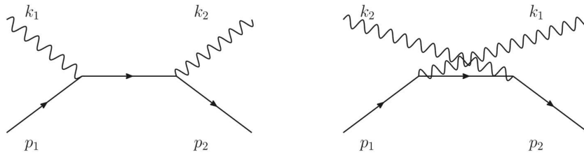
Fig. 9. Feynman diagrams for the Compton effect in the second order
