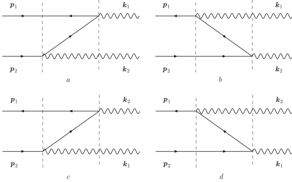
Fig. 6. The direct (a, b) and exchange (c, d) OFPT diagrams for interaction (46)
