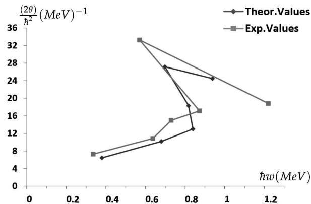
Fig. 3. Inertia moments as a function of the rotational energy for even 60 Fe isotope
