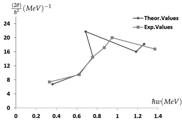
Fig. 2. Inertia moments as a function of the rotational energy for even 58 Fe isotope
