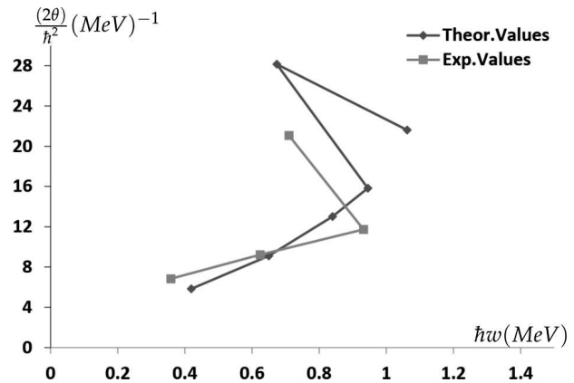
Fig. 4. Inertia moments as a function of the rotational energy for even 62 Fe isotope
