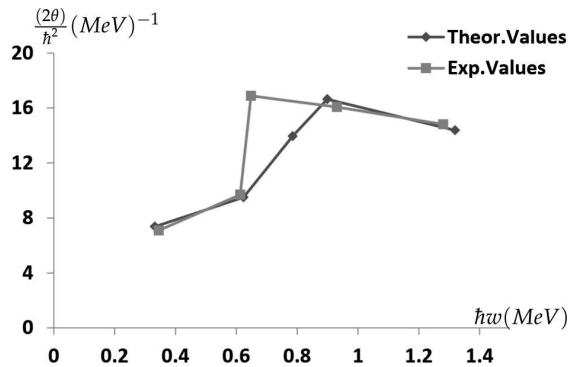
Fig. 1. Inertia moments as a function of the rotational energy for even 56 Fe isotope
