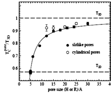
Fig. 3. Size dependence of the pore critical temperature (computer experiment [82])
