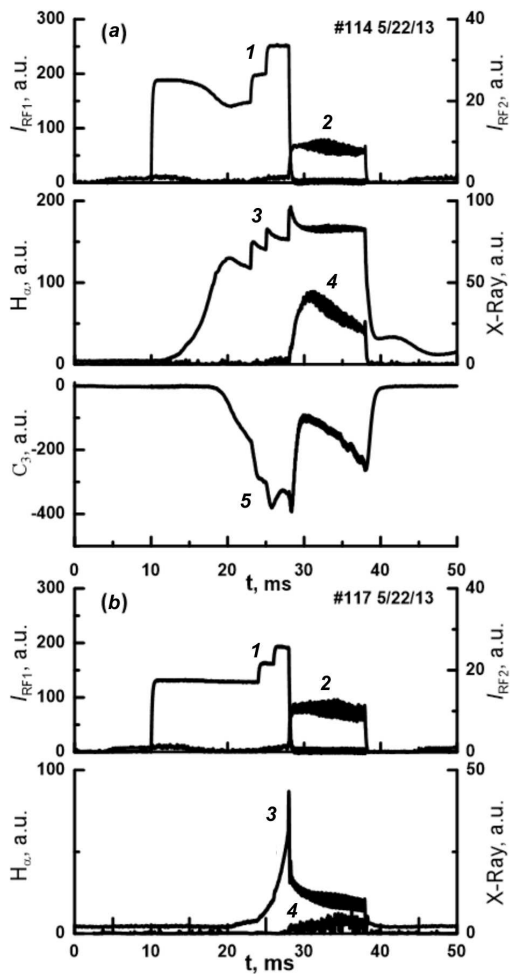
Fig. 2. Temporal behavior of currents fed to the RF antennas of generators – 1 and 2; glow of the H_{\alpha} line and X-ray signal – 3 and 4; glow of the C_3 line – 5. Case (a) – with microwave stimulation at the front edge of the magnetic field pulse and (b) – without microwave stimulation
