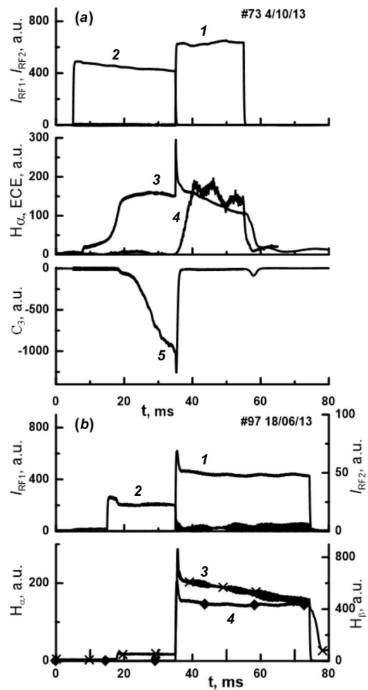
Fig. 3. Temporal behavior of currents fed to the RF antennas – 1 and 2; glow of the H_{\alpha} line and the electron cyclotron emission signal – 3 and 4 (a); glow of the H_{\alpha} and H_{\beta} lines – 3 and 4 (b); glow of the C_3 line – 5 (a)
