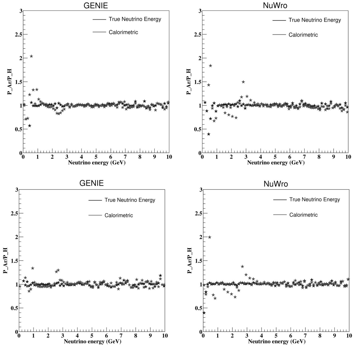
Fig. 8. Ar/H Ratio of Muon (anti)neutrino survival probability as a function of reconstructed neutrino energy represented by red Calorimetric method, and as a function of true neutrino energy represented by blue lines for \nu_\mu (top) and \bar{\nu}_\mu (bottom) from GENIE and NuWro in the left and right panels, respectively
