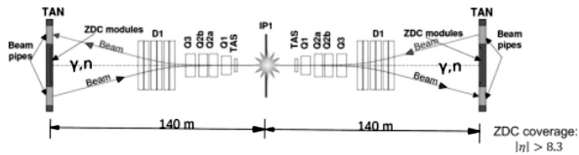
Fig. 3. Diagram of the ATLAS experiment setup including the Zero Degree Calorimeter (ZDC) for detecting \gamma N events in ultraperipheral collisions [2]
