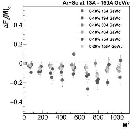
Fig. 1. Summary of published proton intermittency results from NA61/SHINE Ar + Sc energy scan. Results on the dependence of the scaled factorial moment of proton multiplicity distribution on the number of subdivisions in cumulative transverse momentum space M^2 for 1^2 \leq M^2 \leq 32^2 are shown. Points for different energies are slightly shifted in the horizontal axis to increase readability
