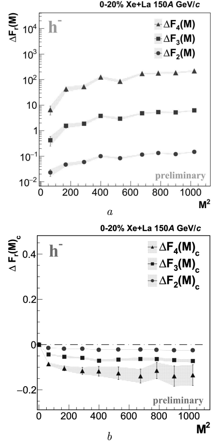
Fig. 2. Negatively charged hadrons intermittency results from NA61/SHINE Xe + La collisions at 150A GeV/c beam momentum. Results on 2nd, 3rd, and 4th scaled factorial moments of negatively charged hadrons multiplicity distribution on the number of subdivisions in p_T binning (a) transverse momentum space 1^2 \leq M^2 \leq 32^2 and in cumulative p_T binning cumulative transverse momentum space (b) are shown. The open circles represent results on 0–20% central Xe+La collisions at 150A GeV/c
