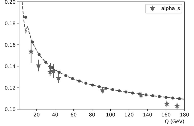
Fig. 4. The expression for \alpha_s as proposed in Eq. (26) is compared with experimental data (green stars) [32]. The red dashes correspond to \Lambda = 100 MeV and values of N_f depending on the opening of the energy threshold, the green dots are for N_f = 5 . The gap corresponds to the threshold N_f = 4 \rightarrow 5
