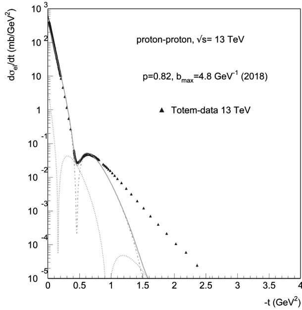
Fig. 2. TOTEM 13 TeV data and the BN model with an exponential cut-off, plot courtesy from A. Grau
