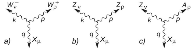
Fig. 2. Vertex diagrams of the interaction of the CS boson with vector fields of the SM in accordance with (3)
