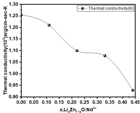
Fig. 8. Thermal conductivity ( k_{min} ) variation in Li_xZn_{1-x}O:Nd^{3+} with dopant concentration
