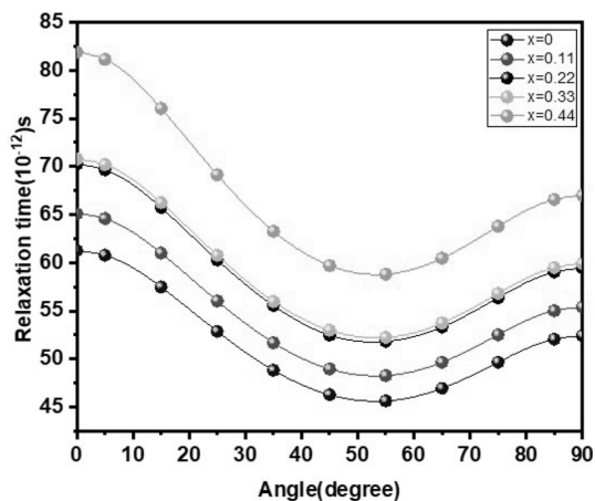
Fig. 10. Variation of angle-dependent relaxation time in Li_xZn_{1-x}O:Nd^{3+} with dopant concentration
