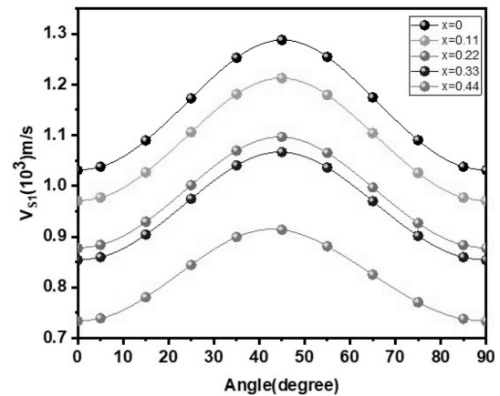
Fig. 5. Variation of angle-dependent ultrasonic velocity ( V_{S1} ) in \text{Li}_x\text{Zn}_{1-x}\text{O}:\text{Nd}^{3+} with dopant concentration
