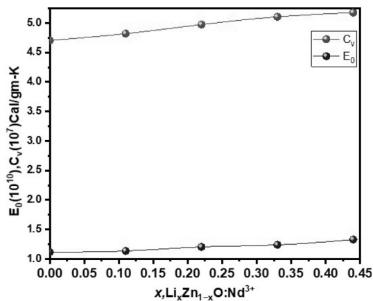
Fig. 9. Variation of the specific heat per unit volume ( C_V ) and energy density ( E_0 ) in Li_xZn_{1-x}O:Nd^{3+} with dopant concentration
