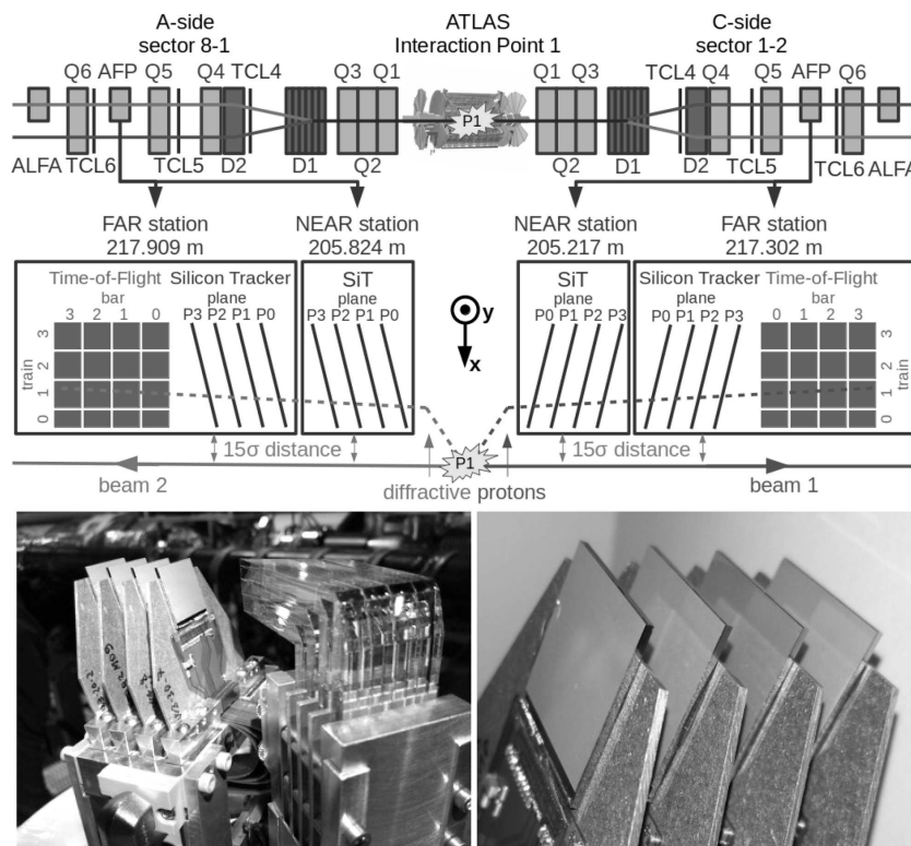
Fig. 11. AFP detector layout and photos of the SiT and ToF detectors
