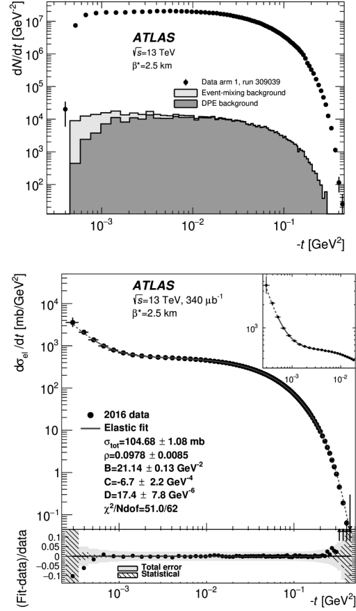
Fig. 7. Mandelstam variable -t distribution and fit (from [2])
