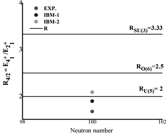
Fig. 1. E(4_1^+)/E(2_1^+) for ^{180}\text{Hg} [27–29]. E(2_1^+) indicate 1 st 2^+ level and E(4_1^+) indicate 1 st 4^+ level. Solid line represented U(5), O(6) and SU(3) limit[1]. The previous data Expt., and those in IBM-1 and IBM-2 are indicated by red, blue, and green colors, respectively
