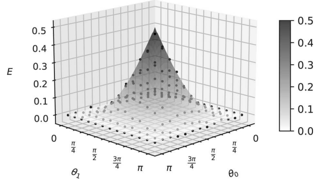
Fig. 6. Results of quantifying the geometric measure of entanglement of qubit q_0 with qubit q_1 in graph state (23) on IBM's simulator Qiskit Aer (marked with dots) and analytical results (represented with a continuous surface)
