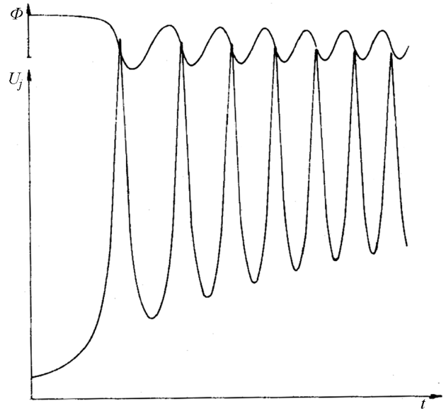
Fig. 1. Stabilization of an explosive instability, from Ref. 4. The oscillations are due to oscillations in \Phi due to an oscillating nonlinear frequency shift. The oscillations in \Phi lead to oscillations in \cos\Phi giving the periodic behavior of the amplitude
