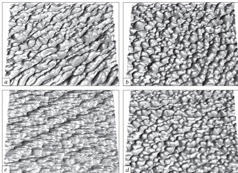
Fig. 4. The 1.0 \times 1.0 \mu\text{m} AFM images of CrN/ZrN coatings with bilayer thickness ( \Lambda ) of 3 \mu\text{m} (a), 375 \text{ nm} (b), 200 \text{ nm} (c), and 100 \text{ nm} (d) [35]
