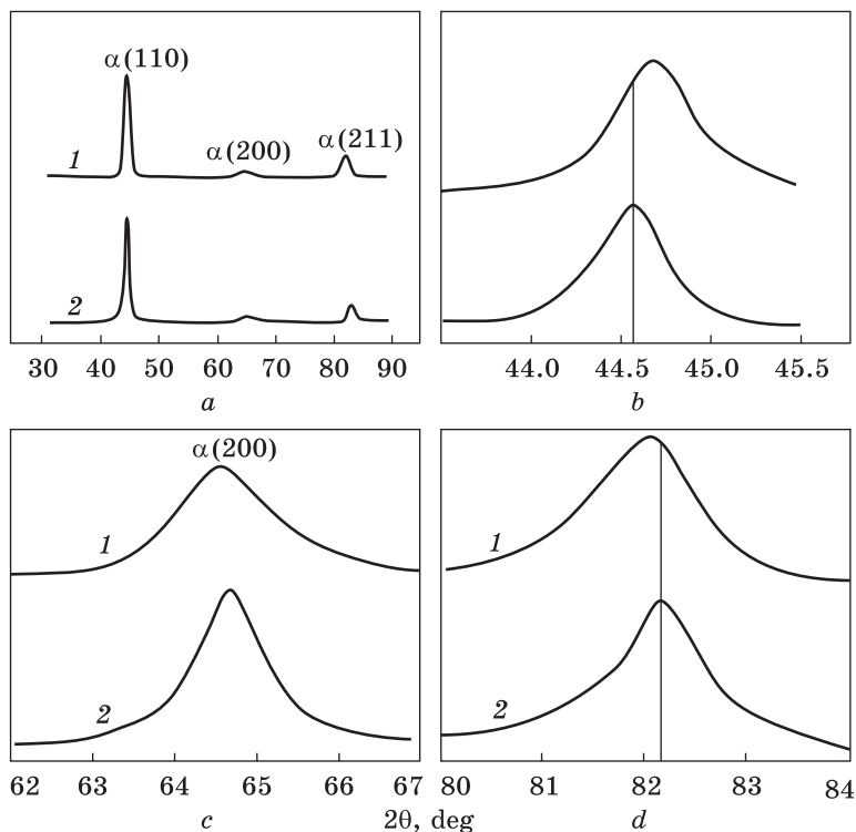
Fig. 24. (a) X-ray spectra for 300M steel: control (2) and US-processed sample (1) and amplified x-ray spectra for control and US-processed sample of (b) \alpha(110) , (c) \alpha(200) and (d) \alpha(211) [21]
