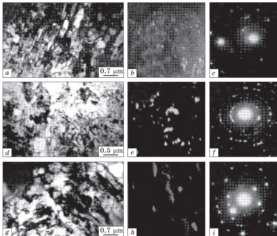
Fig. 5. TEM image of the steel 60 at the depth of 3–4 \mu\text{m} : a, d, g — bright field image; b — dark field for reflex [121] \text{Fe}_3\text{C} ; e — dark field for reflexes [011] \alpha\text{-Fe}^+ [201] \text{Fe}_3\text{C} ; h — dark field for reflexes [011] \alpha\text{-Fe}^+ [031] \text{Fe}_3\text{C} ; c, f, i — micro-electronograms for photo a, d, g , respectively. Steel structure at depth: \sim 3 \mu\text{m} ( a, f ); \sim 5 \mu\text{m} ( g, i ) [12]
