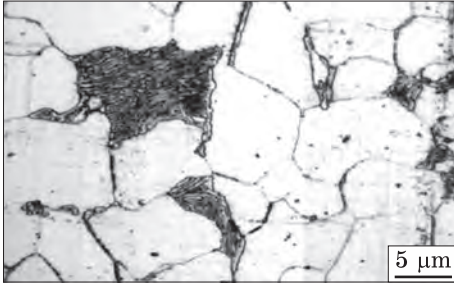
Fig. 16. Optical image of the original structure [19]
