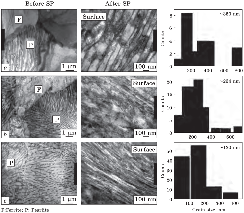
Fig. 48. Cross-sectional TEM — images covering the distance from the top surface to 1 μm below the surface and the grain size distribution along the distance (1 μm). The exposure time was 60 s for (a) 0.1% C, (b) 0.45% C, and (c) 0.8% C steels [37]
