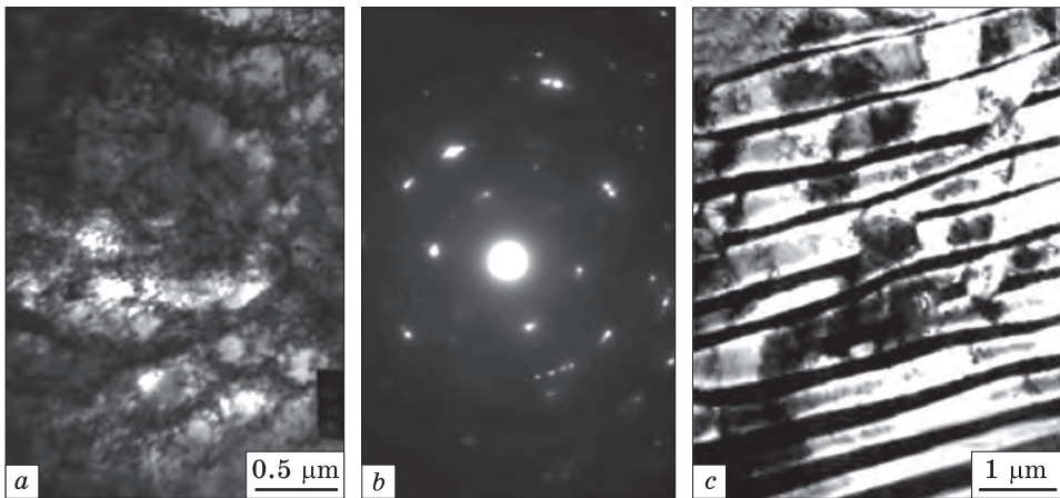
Fig. 29. TEM observations in the subsurface layer microstructure at a depth of 15–25 \mu\text{m} from the outmost surface after HFIP-treatment: the bright field image of the ferrite constituent (a), appropriate SAED pattern (b) obtained from (a), and the pearlite constituent (c) [22]
