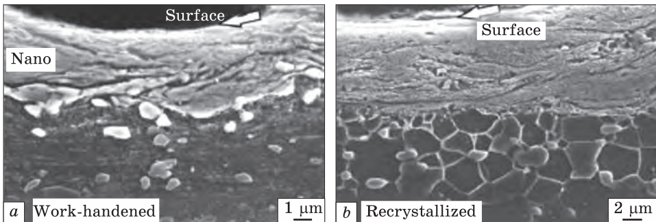
Fig. 38. SEM micrographs of the nanocrystalline regions formed in prestrained (82% cold rolling) Fe-0.80C specimen with spheroidite structure by shot-peened for 10 s. ( a ) As shot-peened and ( b ) annealed at 873 K for 3.6 ks after shot peening [26]
