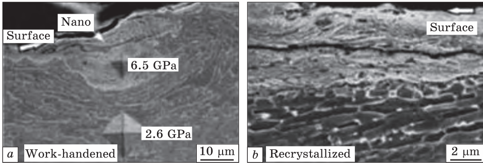
Fig. 37. SEM micrographs of Fe-0.05C-1.29Mn high tensile strength steel after SP for 10 s. a — after SP, and b — annealed at 873K for 3.6 ks after SP [26]
