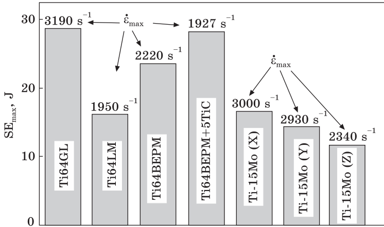
Fig. 18. Comparison of SE max and \dot{\epsilon}_{max} values for Ti-15Mo in the state #2 tested in three mutually perpendicular directions as compared with the data for Ti64GL, Ti64LM (adopted from Ref. [16]), Ti64BEPM, and Ti64BEPM + 5TiC (adopted from Ref. [17])
