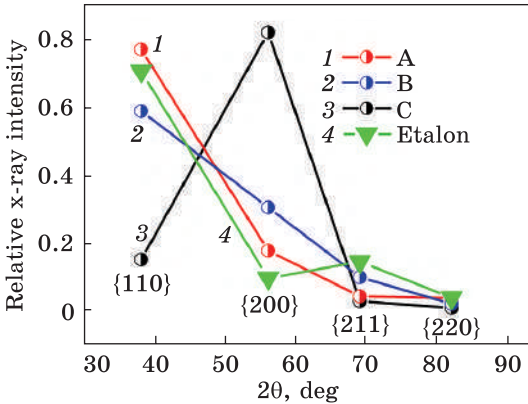
Fig. 15. Relative intensities of reflexes vs. 2θ angle for the planes A, B, C, and for reference β-Ti with random texture
