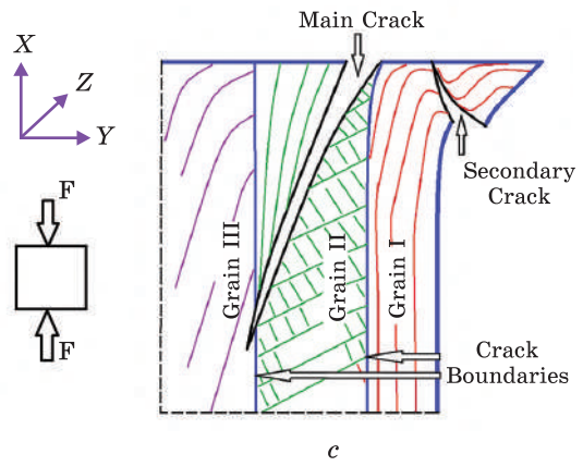
Fig. 20. Schematic presentation of the \beta -grains' shape in the initial state (a). Influence of initial \beta -grains' spatial orientation ( I ) with respect to the applied compressing force ( F ) on the mode of their deformation upon testing ( II ) along the X (b), Y (d), and Z (f) axes. The crack nucleation sites under the compression along X (c), Y (e), and Z (g) axis
