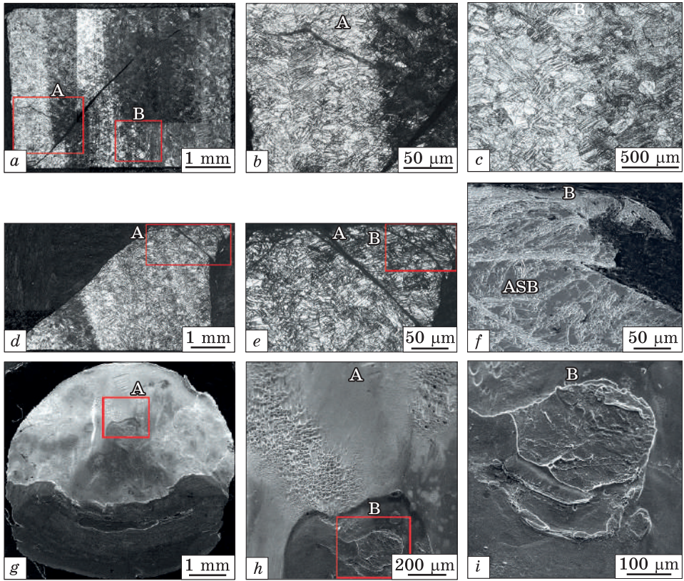
Fig. 13. Microstructure of Ti-15Mo alloy after the SHPB experiments for Y axis orientation with strain rates of 2930 \text{ s}^{-1} ( a ) and 3280 \text{ s}^{-1} , where a – e — LM images, and f – i — SEM images
