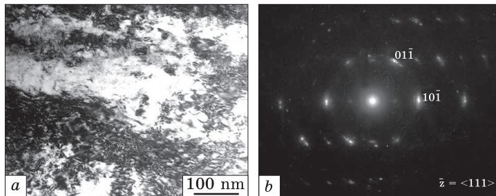
Fig. 10. TEM images of Ti-15Mo tensile tested specimen in the zone 3 (from Fig. 7, d, e), where a — bright field image, b — selected area diffraction pattern
