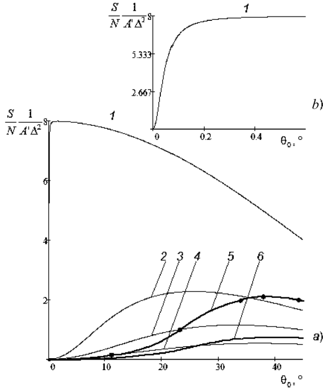
Fig. 4. Dependence \frac{1}{A' \Delta^2} \times \frac{S}{N}(\theta_0) at P = 1 (1), 0.9 (2), 0.7 (3), and 0.5 (4)
