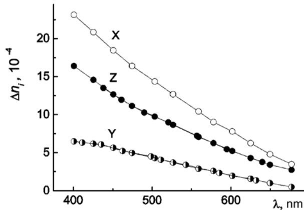
Fig. 2. Dispersion of a birefringence in LiNH 4 SO 4 crystals of the α-modification at room temperature
