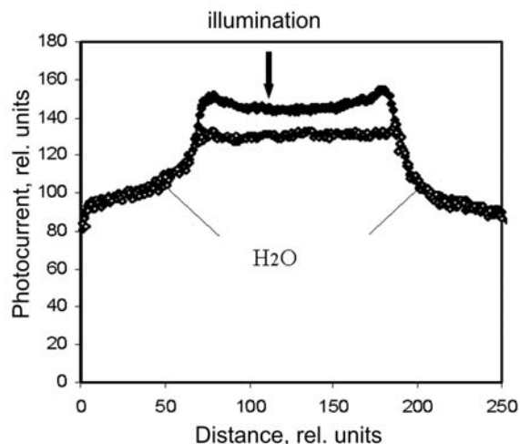
Fig. 6. Distributions of the photo-induced current in a structure with interdigitated back contacts that contacts with distilled water under a permanent illumination with a blue light-emitting diode (solid circles) and without illumination (hollow circles)
