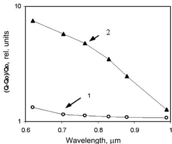
Fig. 5. Relative enhancement of the spectral sensitivity for a structure with interdigitated back contacts when contacting with distilled water (1) and under the permanent illumination with a light-emitting diode (2)
