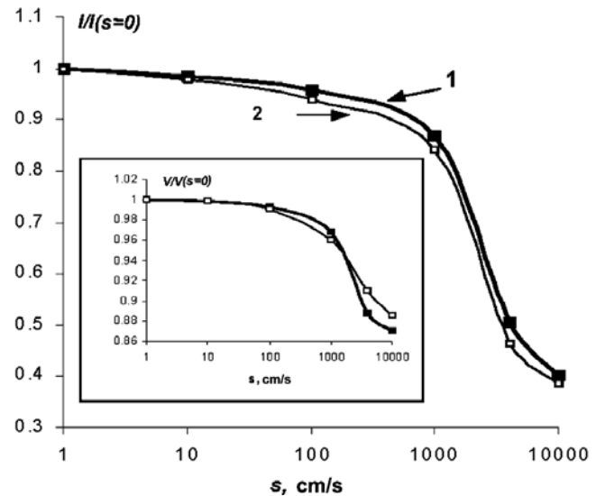
Fig. 4. Calculated dependences of the short-circuit current and the open-circuit voltage (in the inset) on the recombination rate at the illuminated surface for a p-n junction with interdigitated back contacts. The diffusion length is 300 (1) and 100 \mu\text{m} (2)
