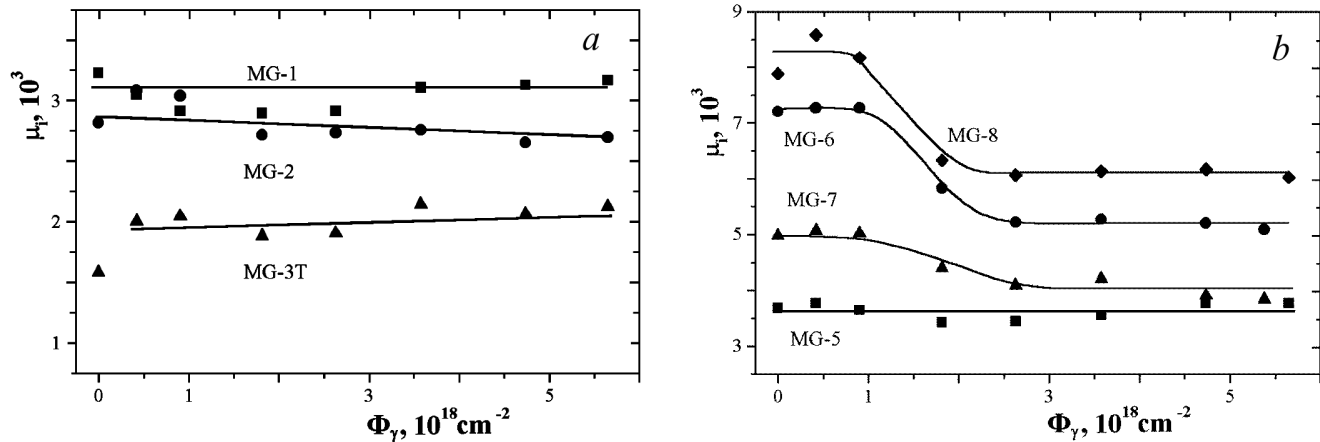
Fig. 1. Dose dependences of the initial magnetic permeability ( f = 10 kHz) of magnetic circuits fabricated from MG-alloys
