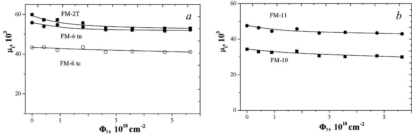
Fig. 2. Dose dependences of the initial magnetic permeability ( f = 10 kHz) of magnetic circuits fabricated from FM-alloys
