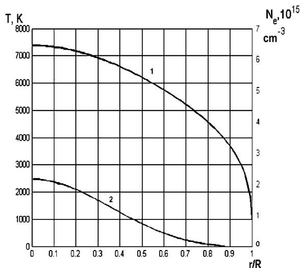
Fig. 1. Radial distributions of the temperature (curve 1) and the electron density (curve 2) in an electric arc with the copper content x_{Cu} = 1\%
