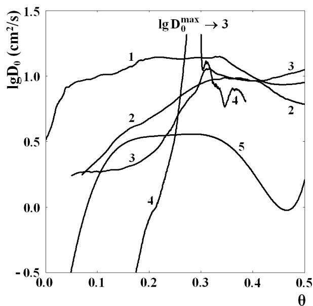
Fig. 9. Dependences of the pre-exponential factor in the Arrhenius equation on the total coverage degree \theta . The notations of curves are the same as those in Fig. 8
