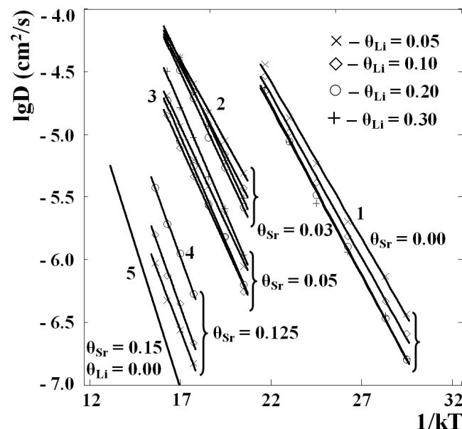
Fig. 7. Arrhenius plots for diffusion coefficients in various adsorption systems: Li-W(112) (1); Li-Sr-W(112), \theta_{Sr} = 0.03 (2); Li-Sr-W(112), \theta_{Sr} = 0.05 (3); Li-Sr-W(112), \theta_{Sr} = 0.125 (4); and Sr-W(112), \theta_{Sr} = 0.15 (5)
