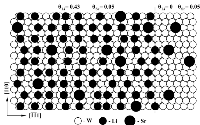
Fig. 1. Diagram of the tungsten (112) face structure. Hollow circles denote tungsten atoms; small and large solid circles denote adsorbed lithium and strontium atoms. \theta_{\text{Li}} \approx 0.43 and \theta_{\text{Sr}} \approx 0.05 . The edge of the lithium concentration stair is marked by a dotted line. The film in the figure is assumed to be structurally noncoherent with the substrate. The long-range order is absent, but the orientational order does take place
