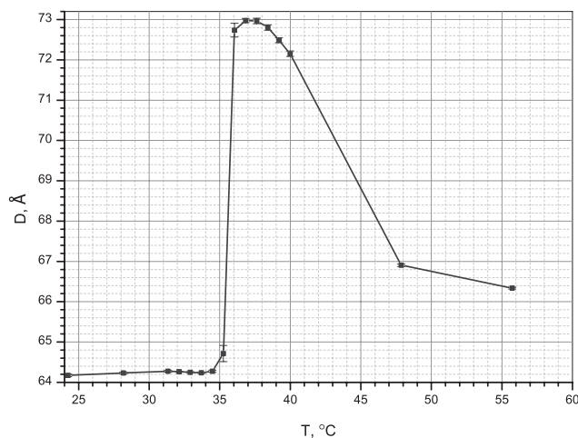
Fig. 3. Temperature dependence of the repetition period of a DPPC lipid bilayer
