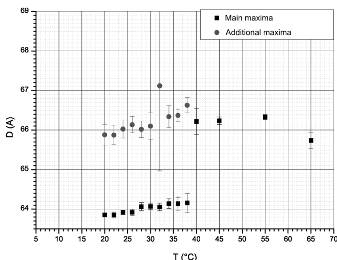
Fig. 6. Temperature dependence of the lipid bilayer repetition period in a lipid mixture DPPC/POPC. Circles and squares denote the repetition periods in the positions of small and main peaks, respectively
