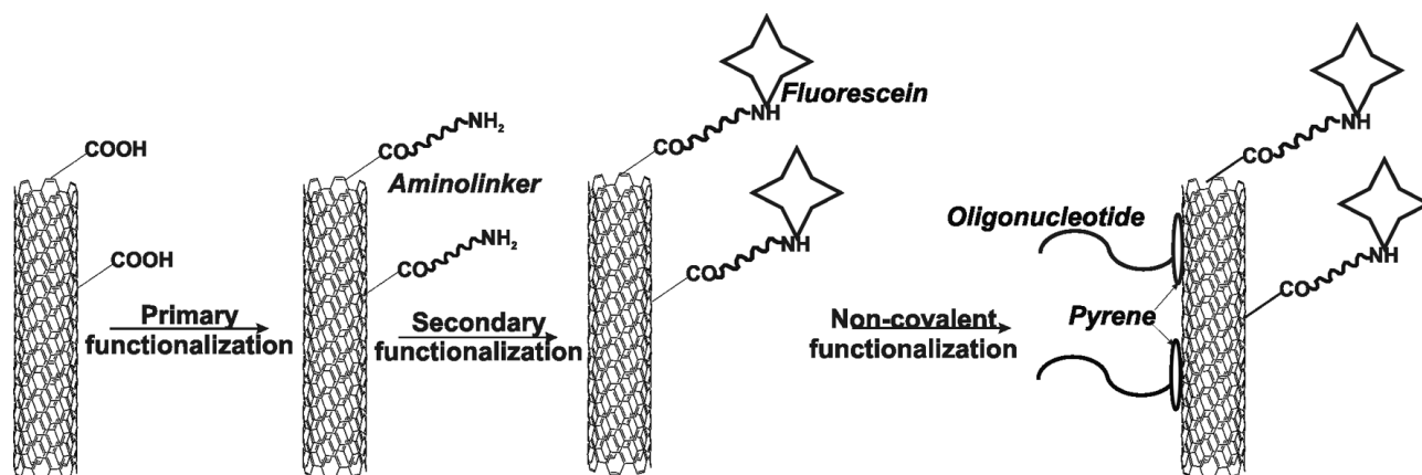
Fig. 1. Strategy of SWNT multifunctionalization
