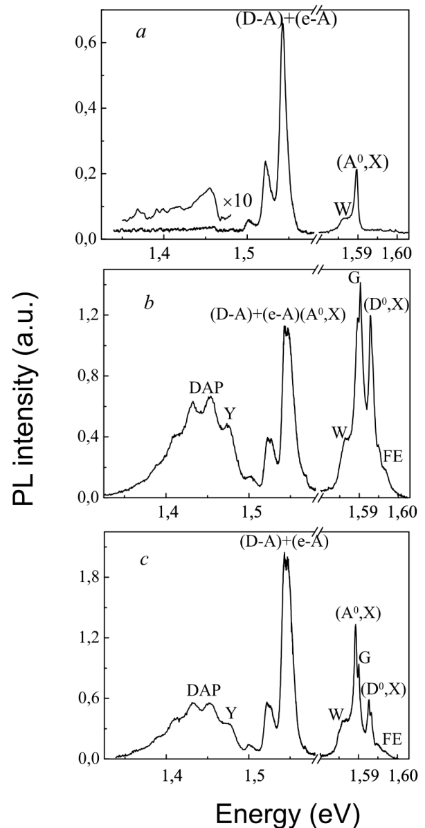
Fig. 1. Typical PL spectra measured at T = 4.5 K for various CdTe specimens grown up by the modified physical vapor transport method: (a) an undoped specimen grown up from the annealed charge, (b) a nominally undoped specimen, and (c) a CdTe:Cl specimen ( N_{\text{Cl}} = 10^{17} \text{ cm}^{-3} ). The spectra in panels (b) and (c) are taken from work [11]
