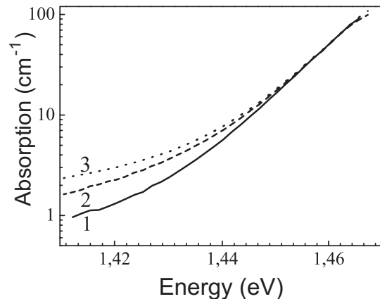
Fig. 2. Spectral dependences of the absorption coefficient measured at T = 300 K for CdTe single crystals in the range of the long-wave intrinsic absorption edge: (1) an undoped specimen grown up from the annealed charge, (2) a nominally undoped specimen grown up from the unannealed charge, and (c) a CdTe:Cl specimen ( N_{\text{Cl}} = 10^{17} \text{ cm}^{-3} )
