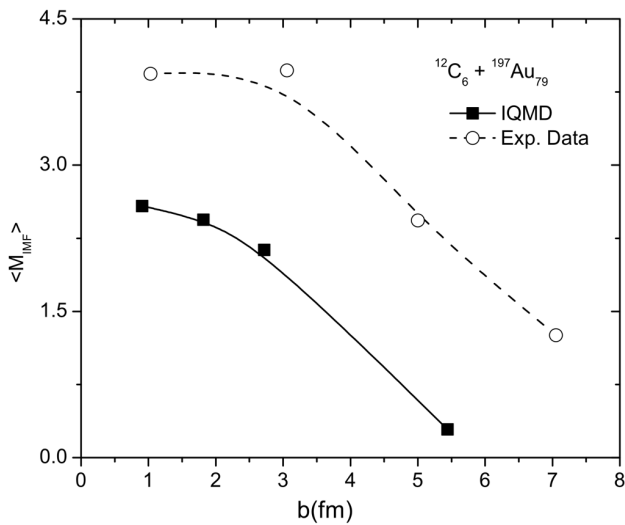
Fig. 4. Mean multiplicity of IMFs vs the impact parameter b , for the experimental data and the IQMD calculations for C + Au at 600 MeV/nucleon
