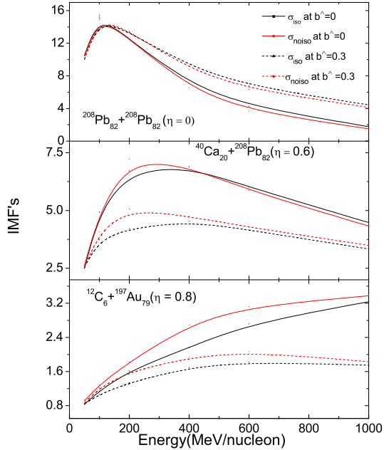
Fig. 2. (Color online) Multiplicity of intermediate mass fragments as a function of energy
