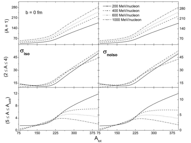
Fig. 3. (Color online) Multiplicity of various fragments vs the total mass of the system ( A_{tot} ) at various energies
