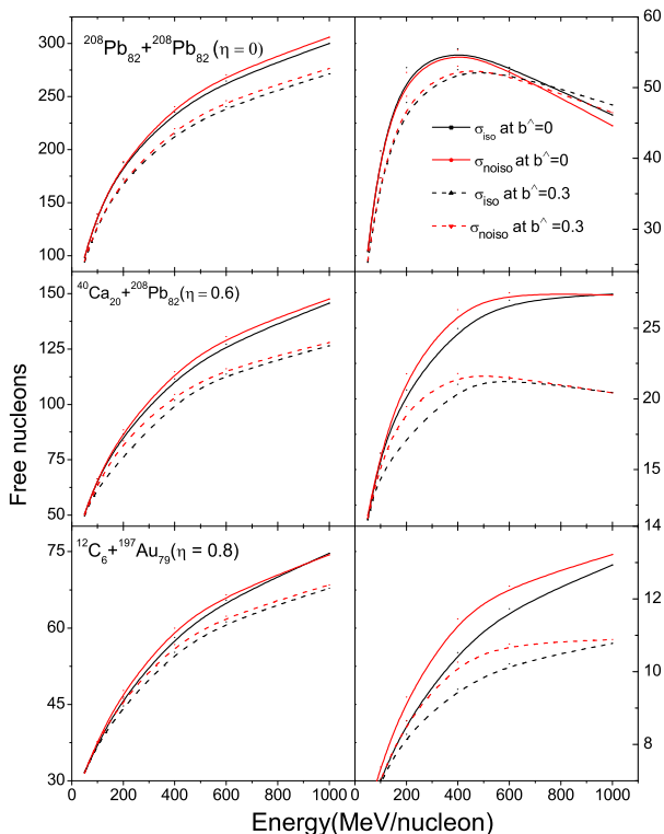
Fig. 1. Multiplicity of free nucleons and LMFs as a function of the energy
