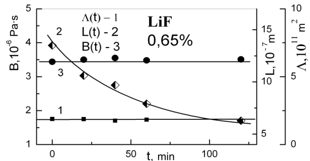
Fig. 4. Dependences of (1) the dislocation density \Lambda , (2) the average effective length of dislocation segments L , and (3) the coefficient of dislocation damping B on the irradiation time of LiF crystals
