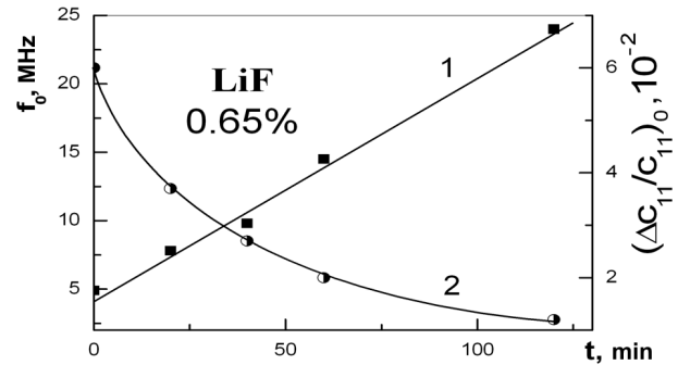
Fig. 3. Dependences of (1) the frequency f_0 and (2) the modulus defect (\Delta C_{11}/C_{11})_0 on the irradiation time of LiF crystals
