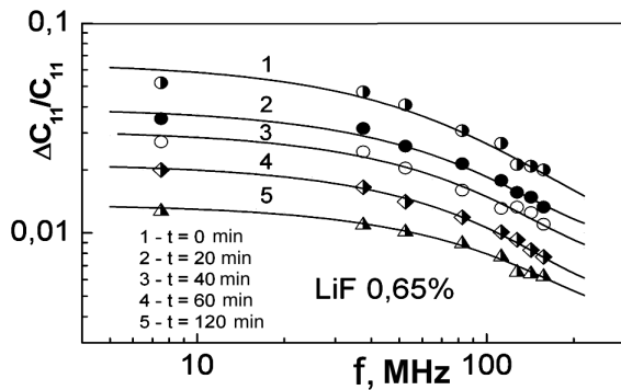
Fig. 2. Frequency dependences of the modulus defect in LiF crystals (1) deformed to 0.65%, and (2 to 5) x-ray-irradiated for 20, 40, 60, and 120 min, respectively. Solid curves are the theoretical curves taken from work [11]
