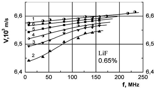
Fig. 1. Frequency dependences of the ultrasound propagation velocity in LiF crystals for (1) a non-strained specimen, (2) a specimen with a residual deformation of 0.65%, and (3 to 6) a specimen deformed to 0.65% and x-ray-irradiated for 20, 40, 60, and 120 min, respectively
