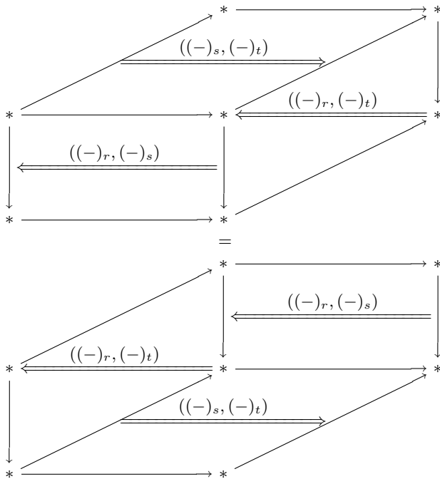
Fig. 1. Cubic relations in the Gray product
