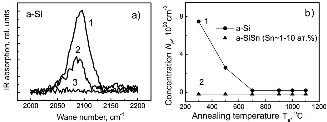
Fig. 2. (a) Spectra of optical density for thin a-Si films: as-deposited at T_s = 300 °C (1) and annealed at temperatures of 500 (2) and 700 °C (3). (b) Dependences of the hydrogen concentration in a-Si films (1) and a-SiSn films with Sn contents within the interval of 1–10 at.% (2) on the temperature of isochronous (for 20 min) annealing
