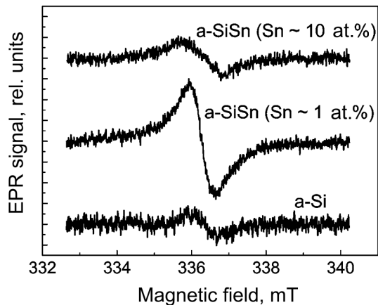
Fig. 3. EPR spectra for as-deposited a-Si and a-SiSn films registered under identical conditions
