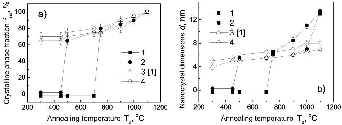
Fig. 1. Dependences of (a) the relative volume fraction of the silicon crystalline phase and (b) the nanocrystal dimensions in the films on the isochronous (for 20 min) annealing temperature: a-Si film (1), a-SiSn films with Sn contents of 1 (2), 4 (3), and 10 at.% (4). Spectrum 3 was obtained in work [1] and is shown for comparison
