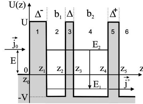
Fig. 1. Energy diagram for of an electron in the 3BRTS with shifted bottoms of potential wells
