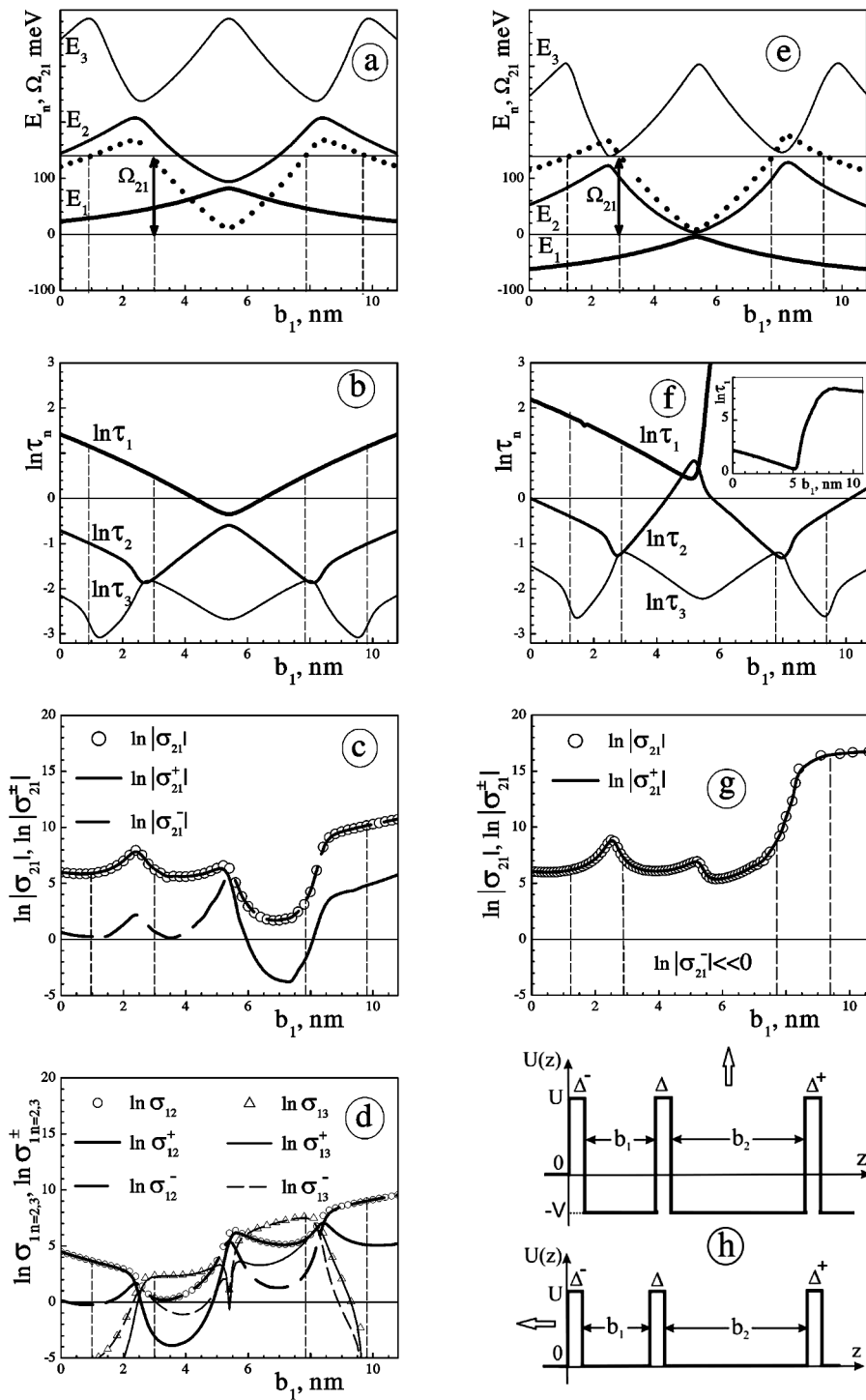
Fig. 2. Dependences of E_n , \ln \tau_n , \ln \sigma_{n,m} , and \ln \sigma_{n,m}^\pm on b_1 for 3BRTSs at V = 0 (a–d) and 100 meV (e–g), and (h) the energy diagrams of those systems
